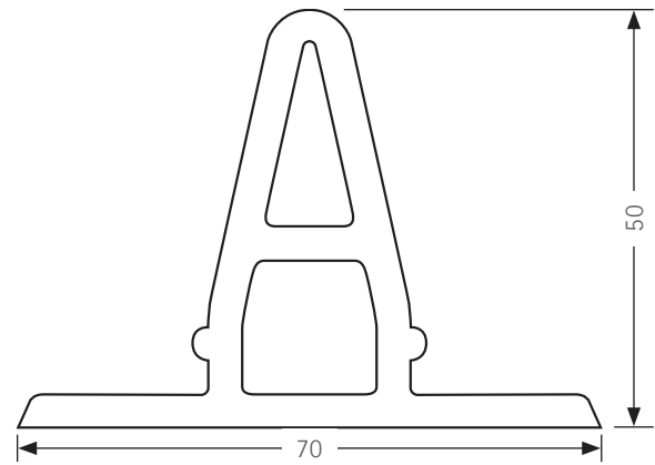
RENOLIT ALKORPLAN Design XL profile X-Large
